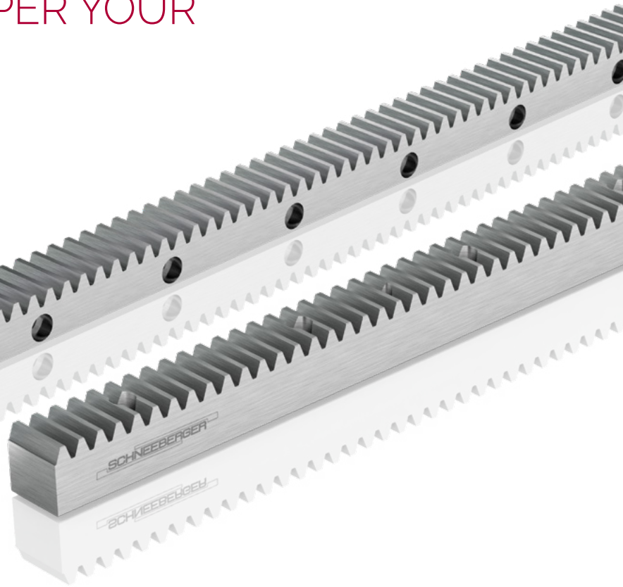
Gear rack with special hole pattern
