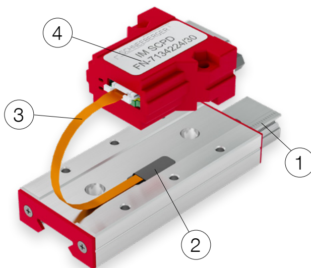
MINISLIDE MSQscale
