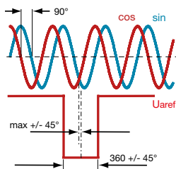
Analogue interface
